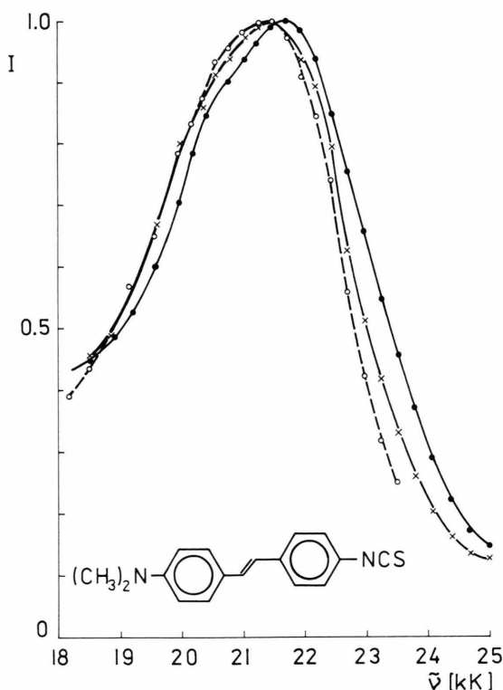
Fig. 1. Fluorescence spectra of CDS in chlorobenzene at 295 K: \nu_{exc} = 28600 \text{ cm}^{-1} (●); \nu_{exc} = 27000 \text{ cm}^{-1} (×); \nu_{exc} = 24400 \text{ cm}^{-1} (○).
